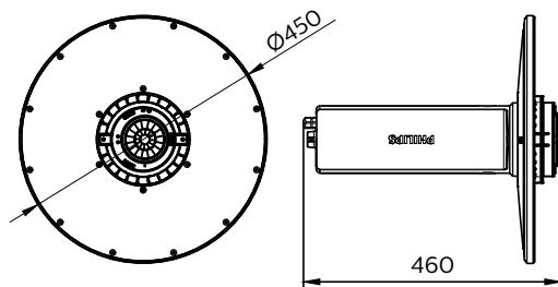
BY718P GreenPerform Highbay Elite
