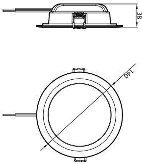
DN020B G3 LED9/NW 10.5W 220-240V D125SNI
